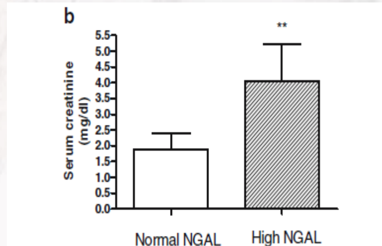
Fig. 2 a Peak BUN concentration during the course of hospitalization in children with D+HUS and normal versus high urinary NGAL excretion. Data are presented as mean \pm SD. * P=0.007 . b Peak serum creatinine concentration during the course of hospitalization in children with D+HUS and normal versus high urinary NGAL excretion. Data are presented as mean \pm SD. ** P=0.01
